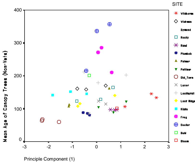
Figure 8. PCA 1 vs mean plot age
