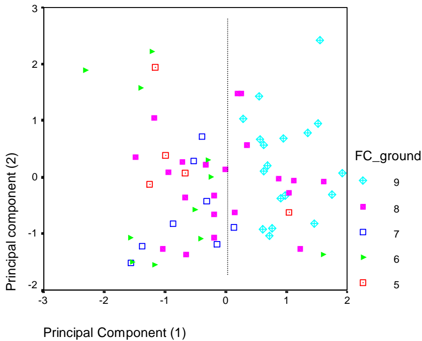
Figure 4. Principal component 1 versus principal component 2, plots marked by measured age class.
