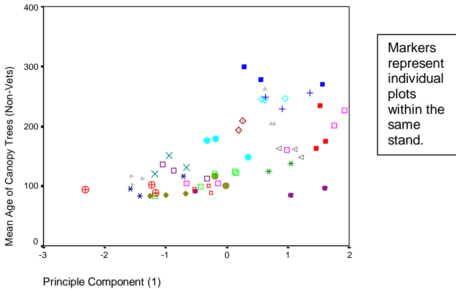
Figure 5. PCA_1 and measured mean age of plots (shown by each stand sampled).
