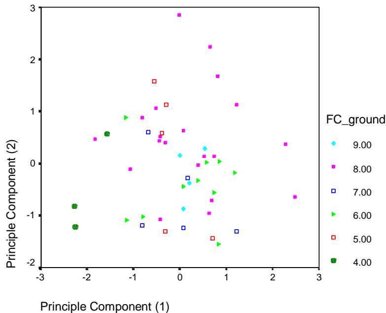
Figure 7. PCA_1 versus PCA_2 for dry MSdk plots
